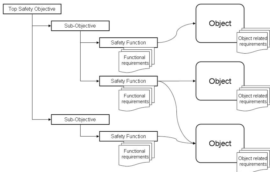
Figure 1 Structure breakdown of functional safety objectives
