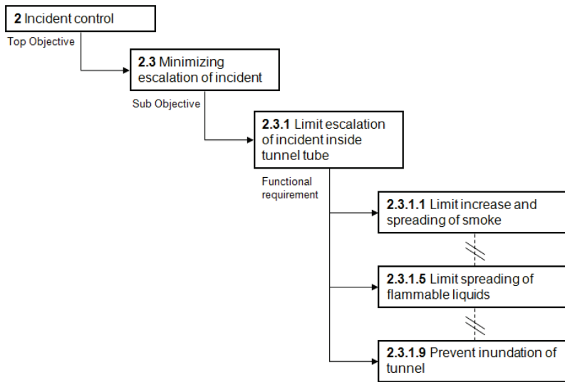
Figure 2 Example of safety structure
